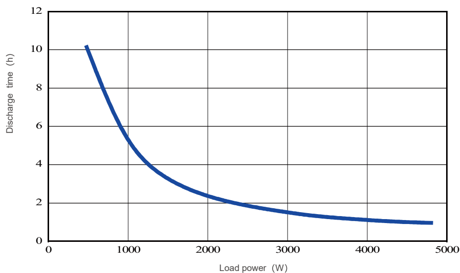
SDA10-48100 Discharge time at different load power
